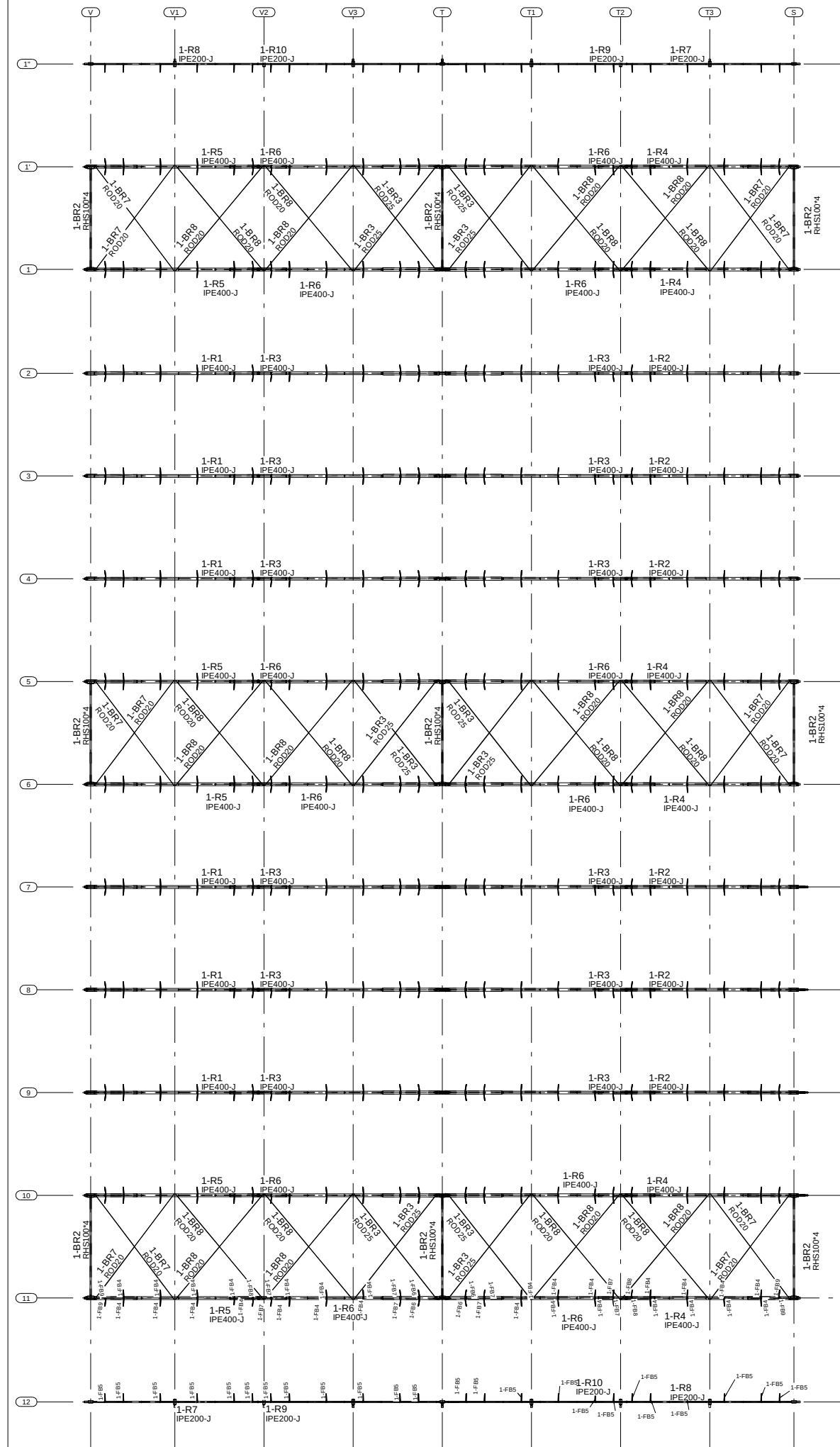
ROOF PLAN WITHOUT PURLIN - Area - 2
